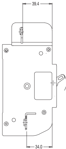
FRONT CONNECTED SCREWTERMINAL
