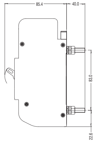
SIDEVIEW BACK CONNECTED STUDS
